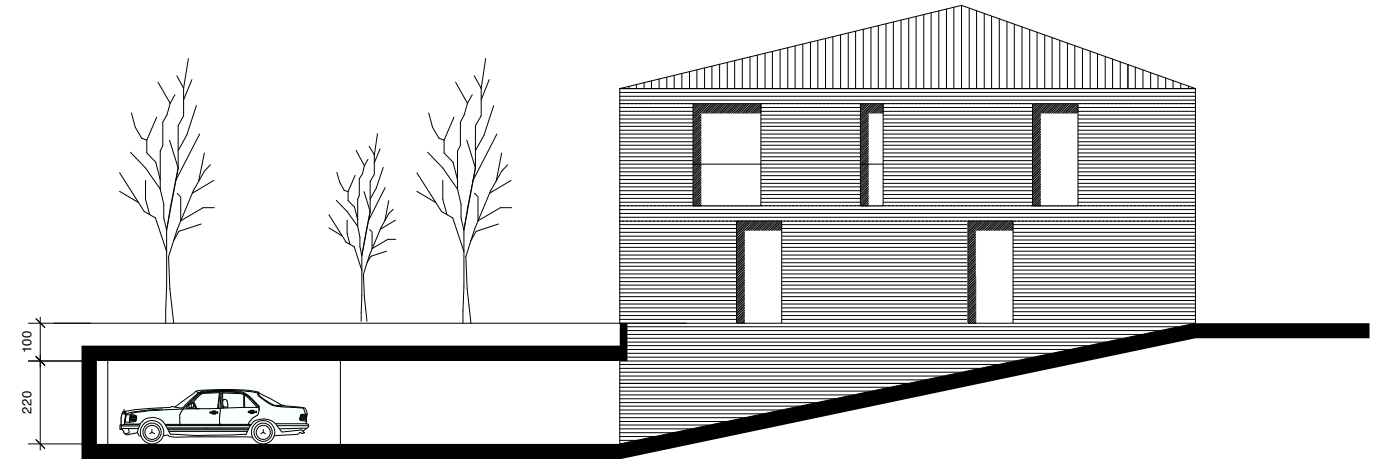
C-C (FRONTE OVEST)
